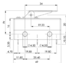
Type 3AS : Simple lever - Indirect Action -
