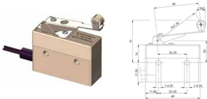
Type 8AL40 : Simple Adjustable Lever with Roller - Direct Action -
