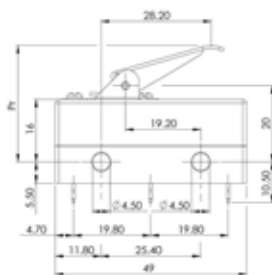
Type 3AS : Simple lever - Indirect Action -
