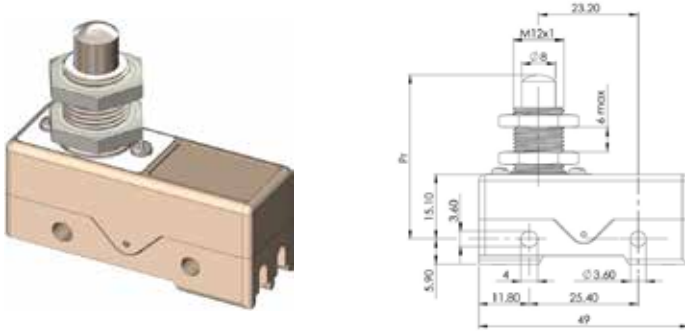
Type 1A58 : Telescopic with Thread
